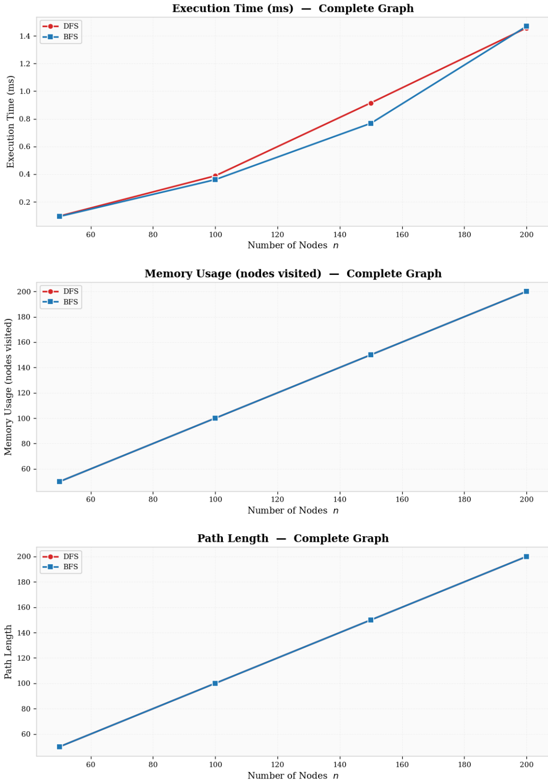
Figure 5: Complete Graph Performance Comparison.
