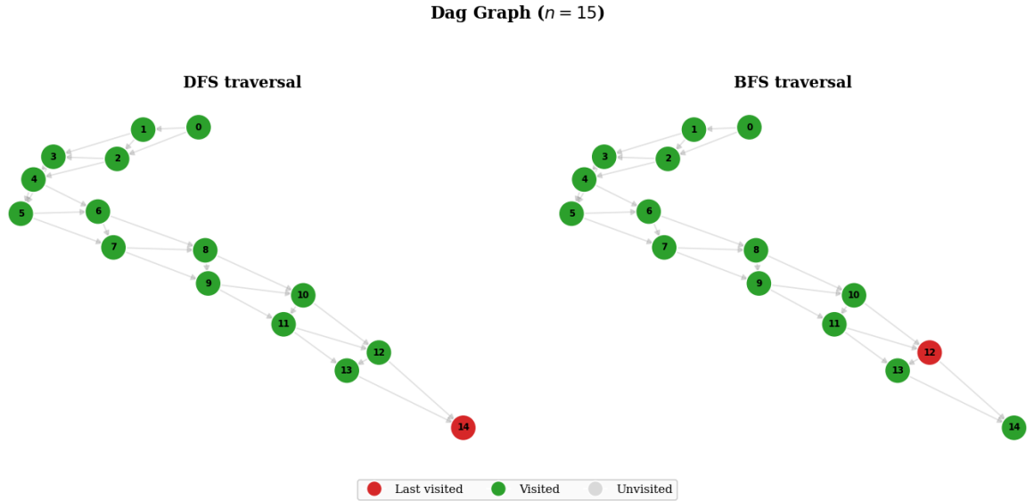
Figure 11: DAG Traversal.
