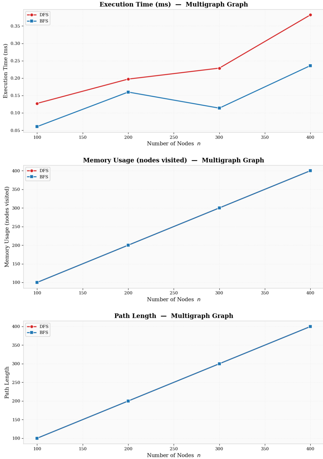
Figure 21: Multigraph Performance Comparison.
