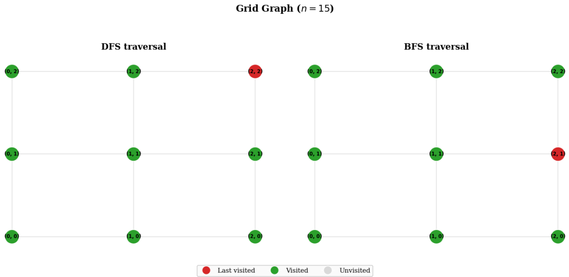
Figure 13: Grid Graph Traversal.
