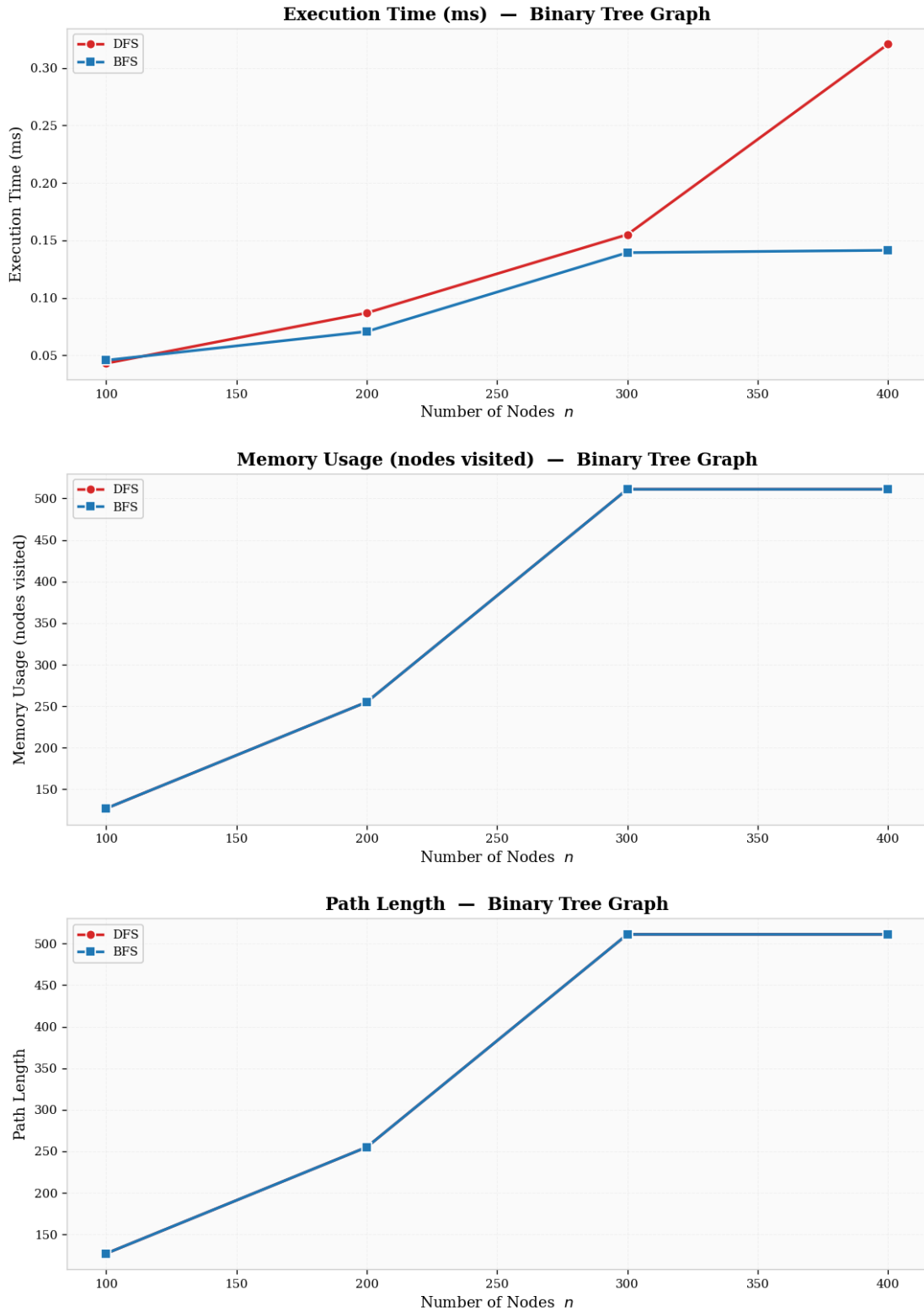
Figure 9: Binary Tree Performance Comparison.
