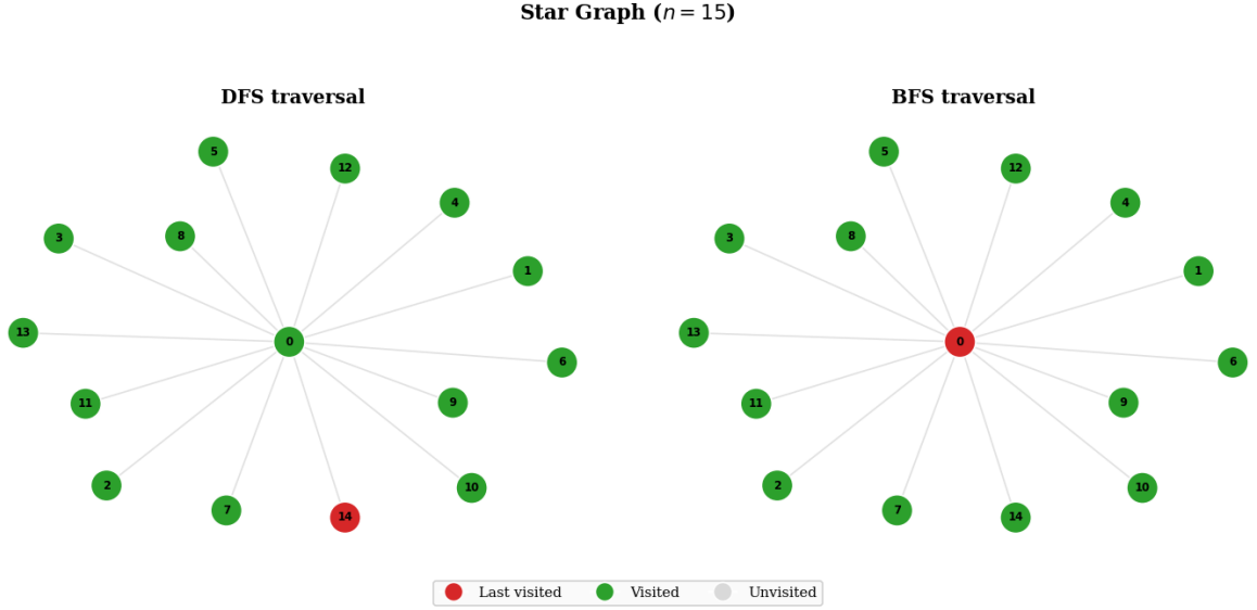
Figure 6: Star Graph Traversal.
