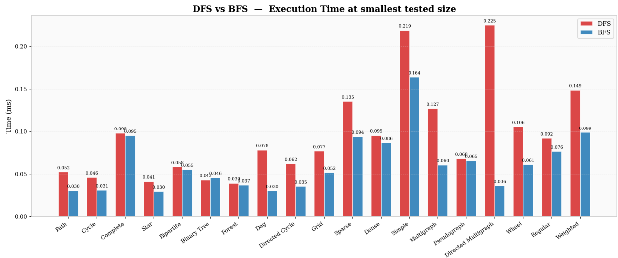
Figure 30: Overall Time Comparison at Tested Size.
