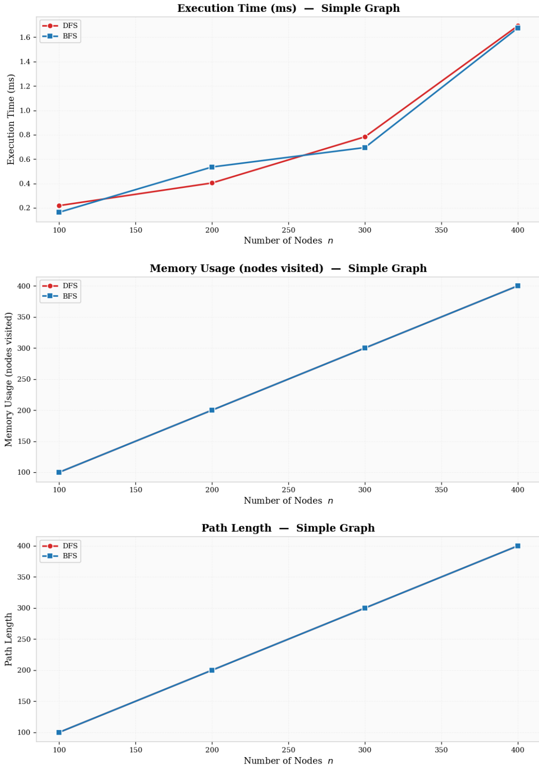
Figure 19: Simple Graph Performance Comparison.
