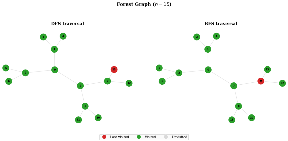
Figure 10: Forest Graph Traversal.
