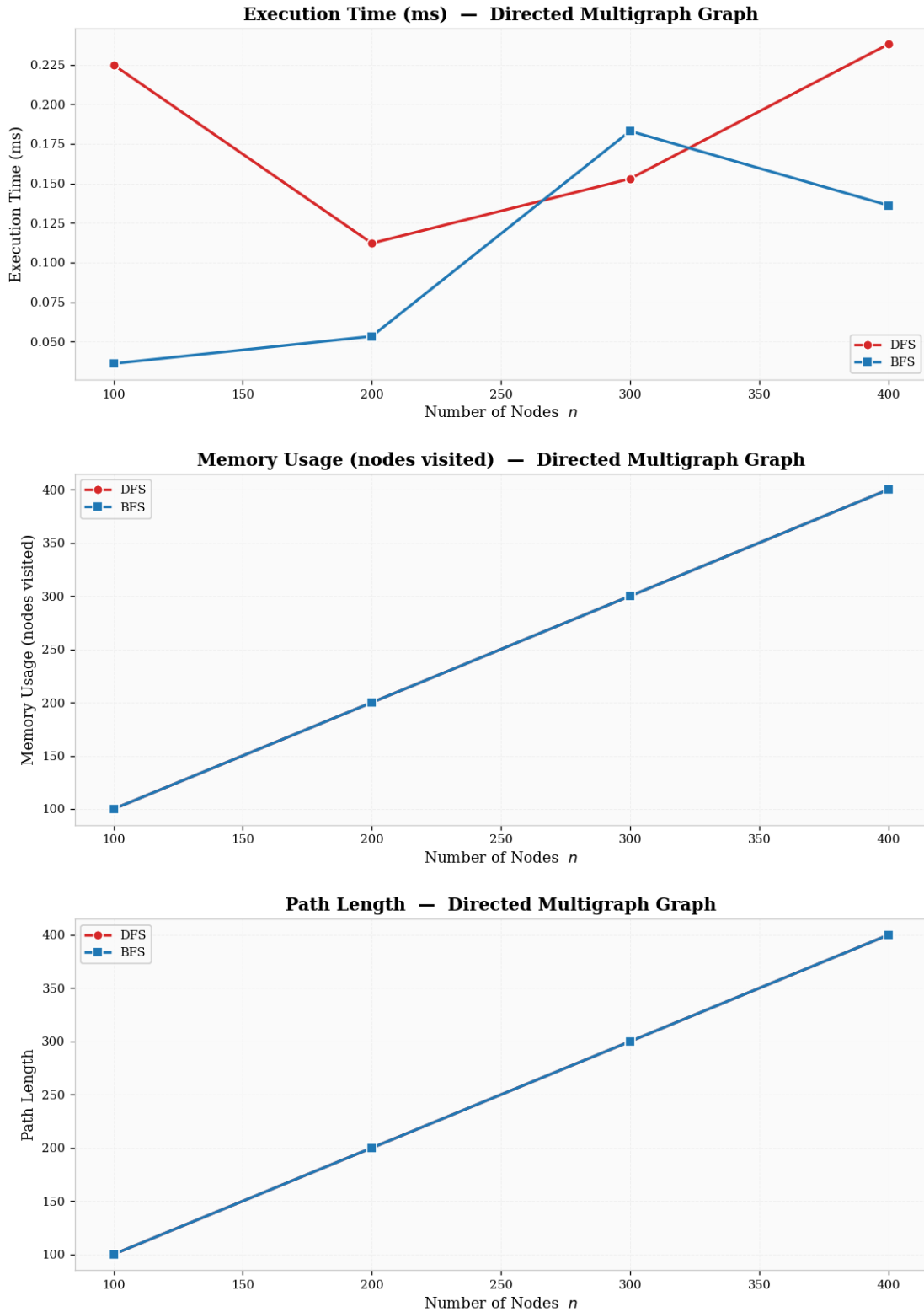
Figure 25: Directed Multigraph Performance Comparison.
