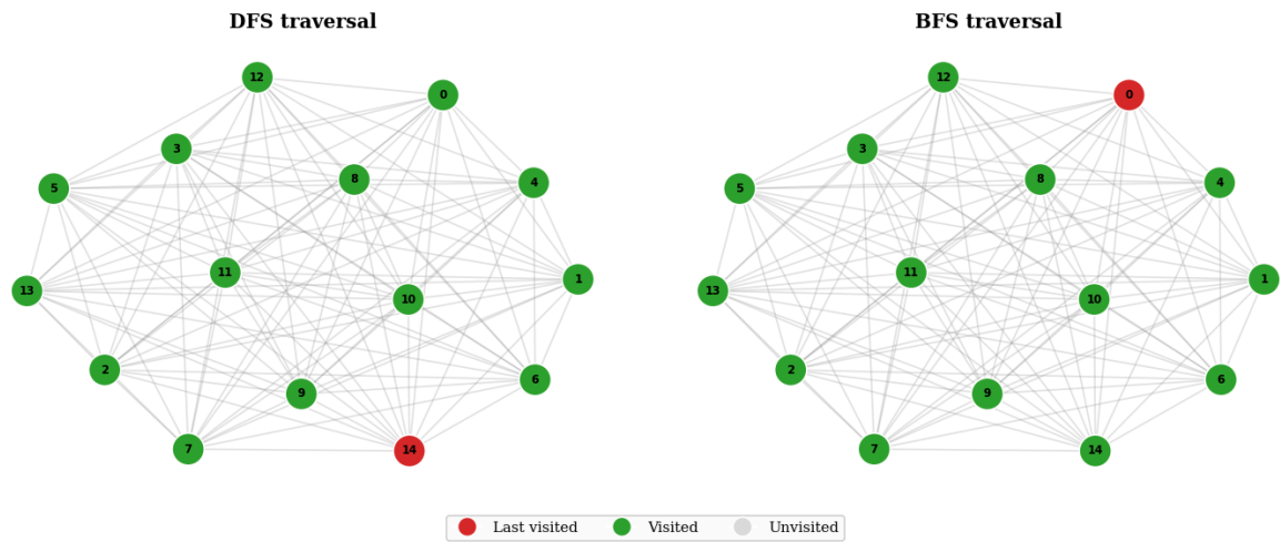
Figure 4: Complete Graph Traversal.
