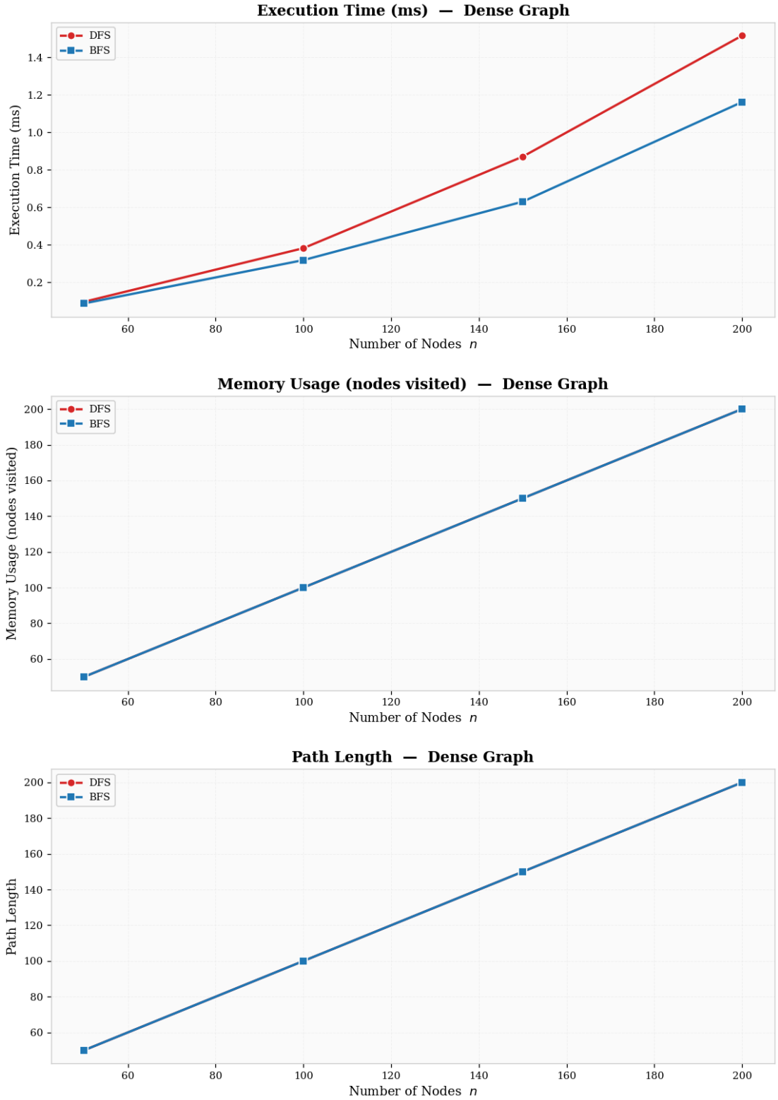
Figure 17: Dense Random Graph Performance Comparison.
