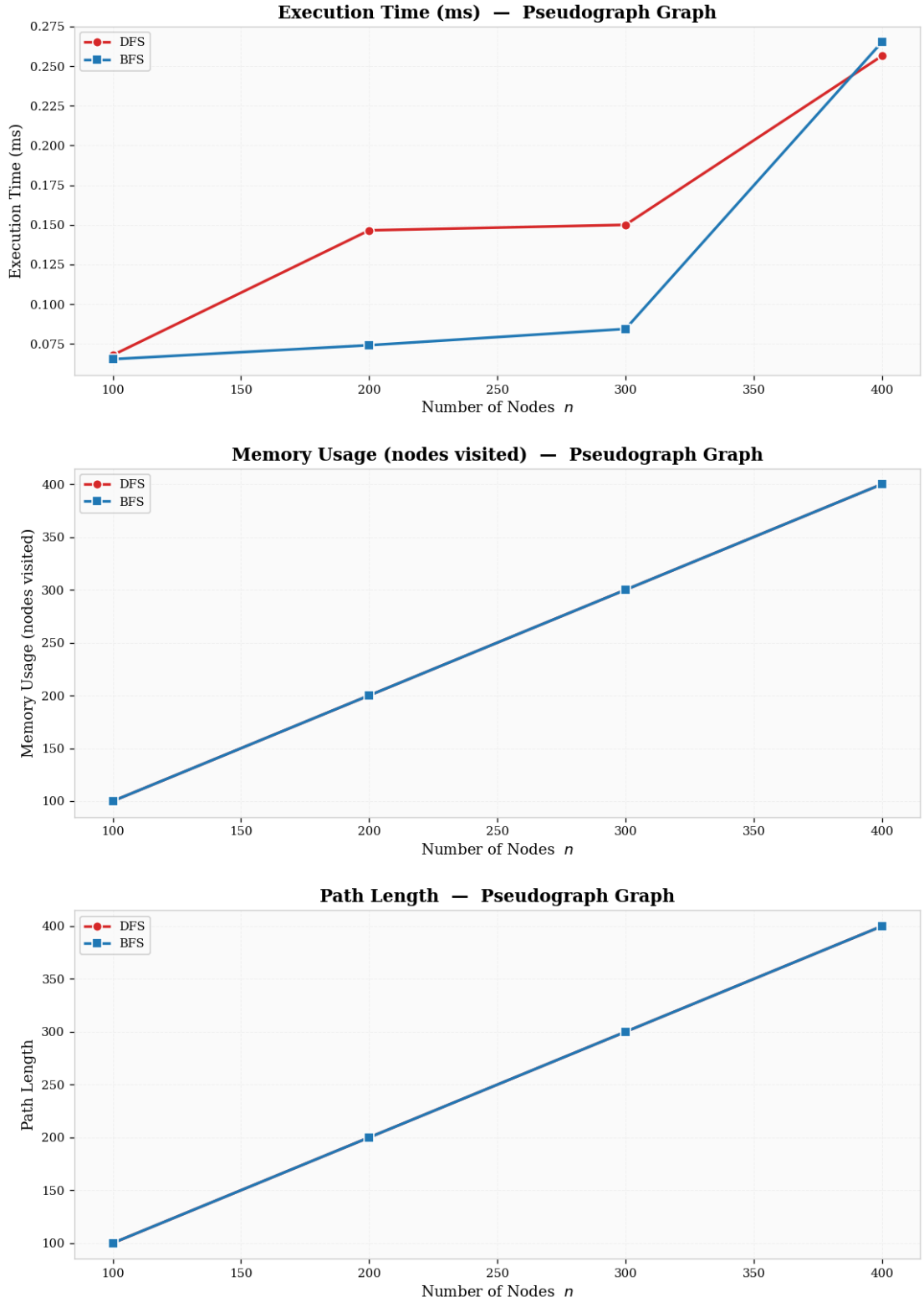
Figure 23: Pseudograph Performance Comparison.
