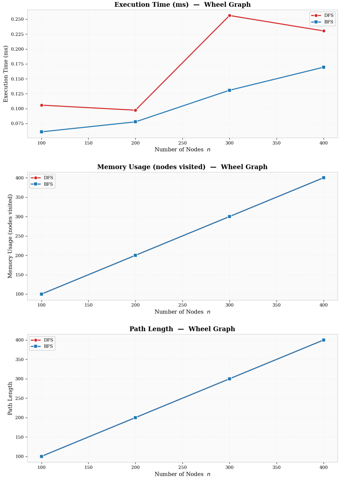
Figure 27: Wheel Graph Performance Comparison.
