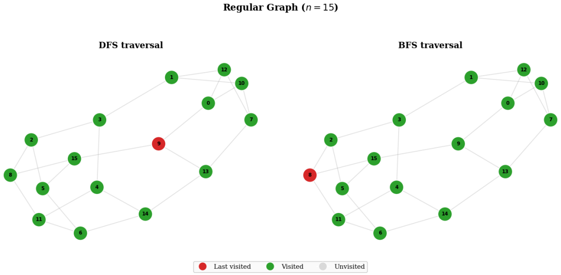
Figure 28: Regular (Cubic) Graph Traversal.
