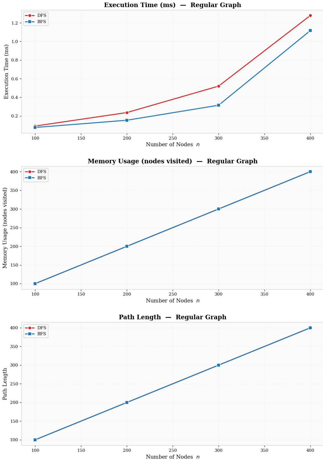
Figure 29: Regular Graph Performance Comparison.
