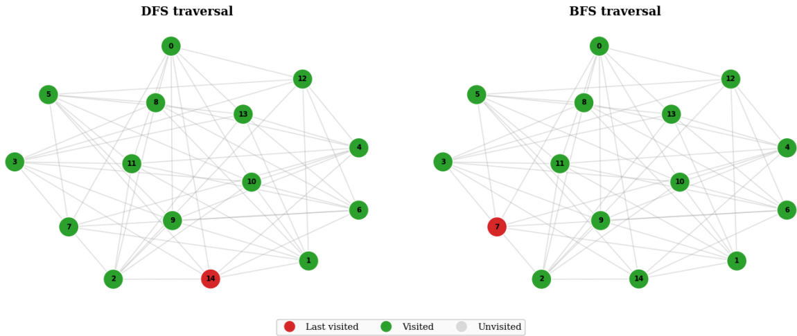
Figure 7: Complete Bipartite Graph Traversal.
