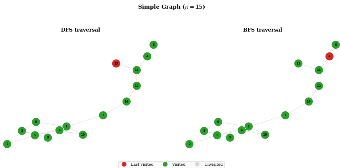
Figure 18: Simple Graph Traversal.
