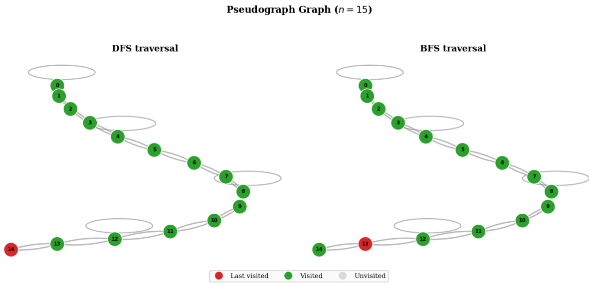
Figure 22: Pseudograph Traversal.
