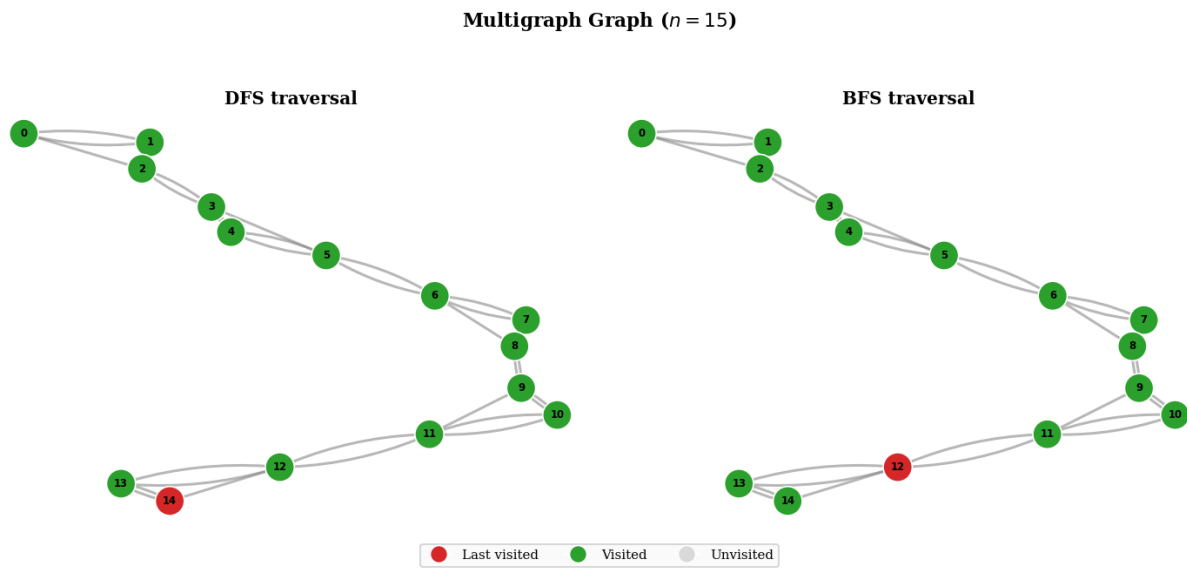
Figure 20: Multigraph Traversal.
