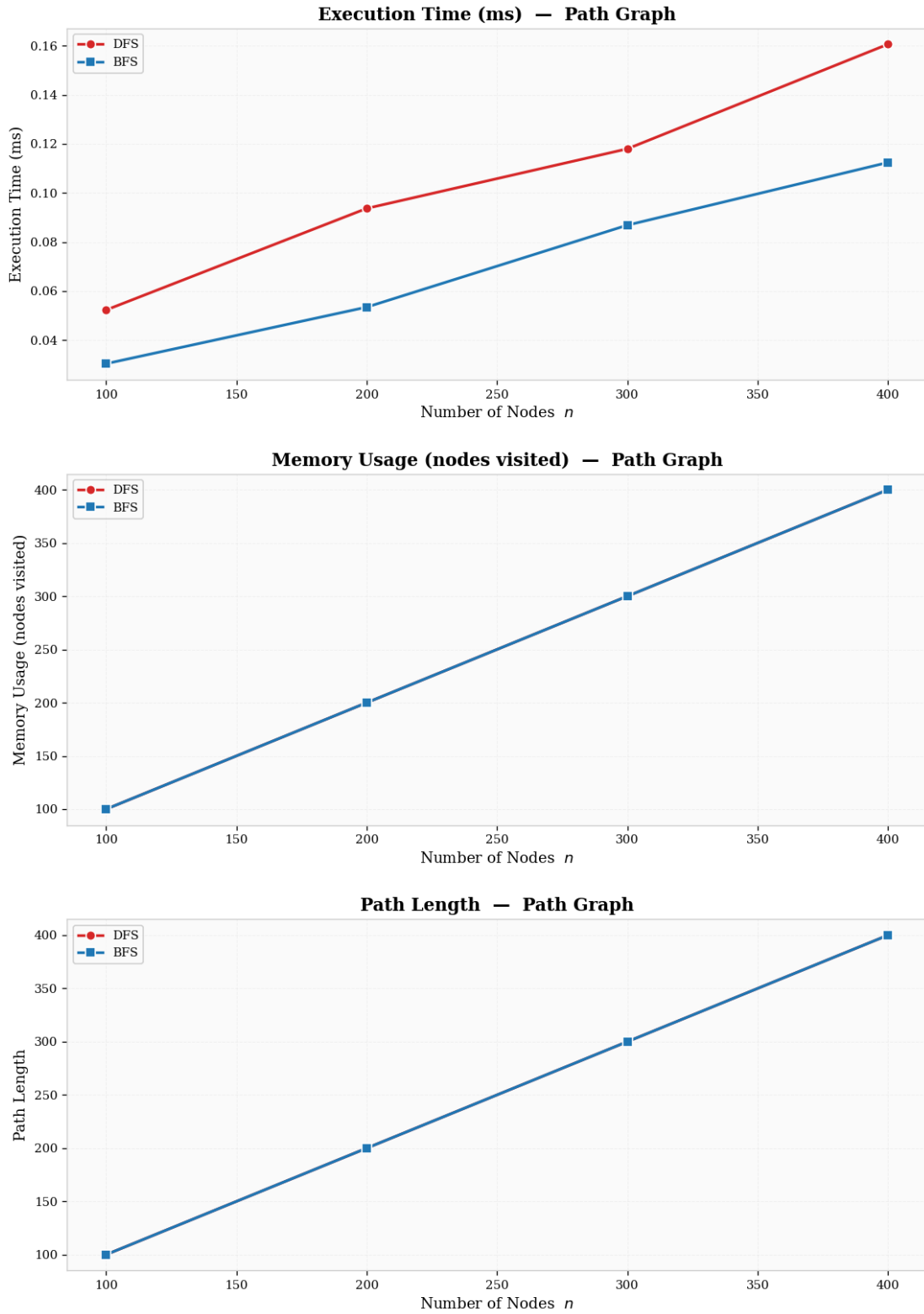
Figure 2: Path Graph Performance Comparison.
