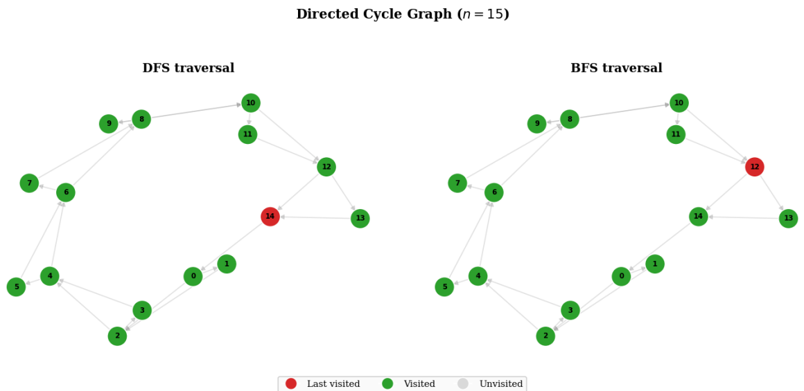
Figure 12: Directed Cycle Traversal.
