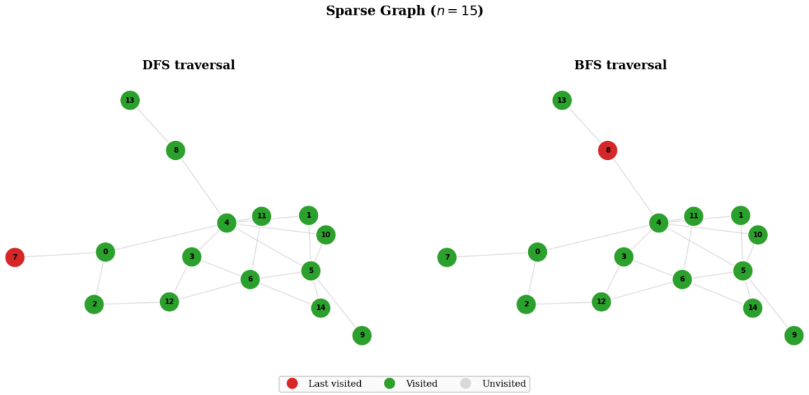
Figure 15: Sparse Random Graph Traversal.
