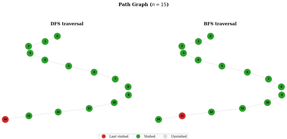
Figure 1: Path Graph Traversal.
