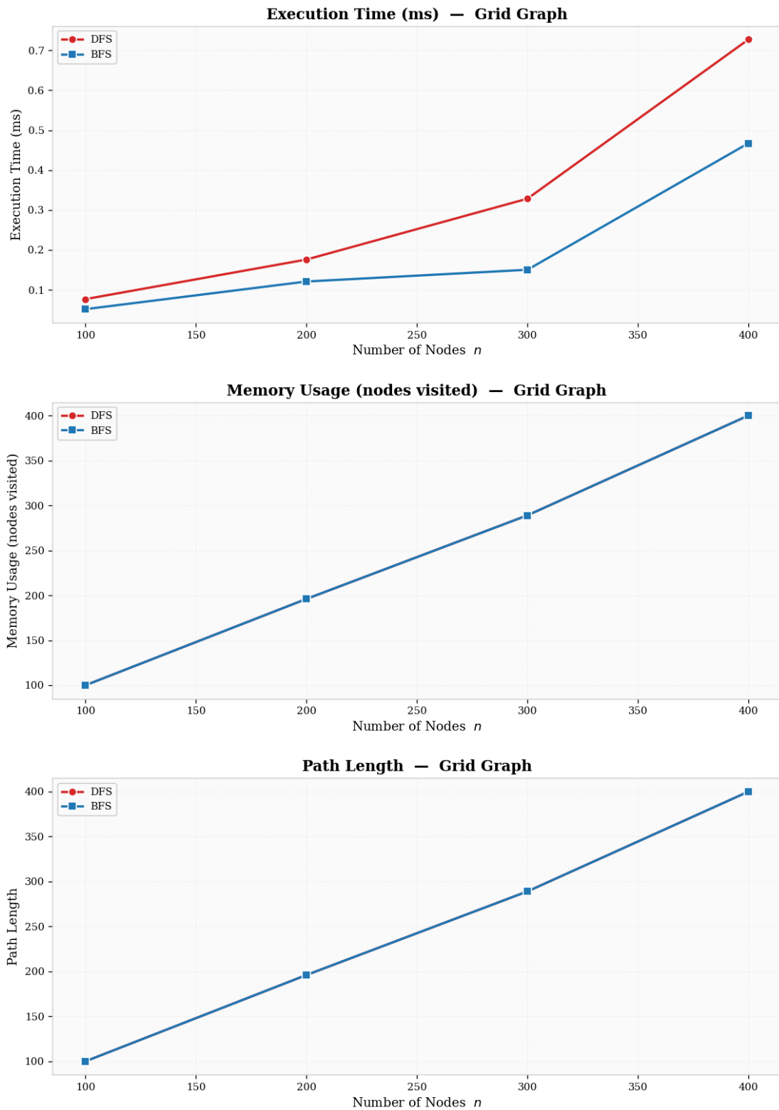
Figure 14: Grid Graph Performance Comparison.
